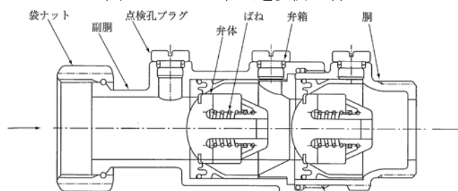
図Ⅱ-13-21 複式逆流防止弁
